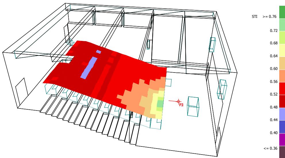
Figure 5 – A grid map showing the STI in the auditorium. The source is a human speaker with vocal effort raised. The results are displayed with the 12-step scale defined in Table 7.
