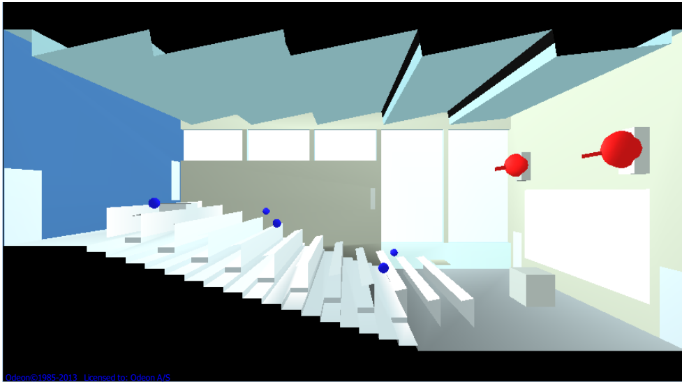
Figure 7 – A view into the model of the auditorium with the sound sources (red) and five receivers (blue).
