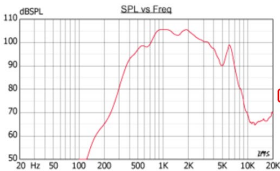
Figure 2 – Example of data sheet for a loudspeaker. This comes in three versions (15W, 20W, 25W) each with six possible tapings. Marked in red: Sensitivity 105 dB SPL 1W/1m and tapping 3W.
