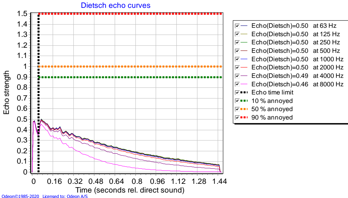
Figure 8: Dietsch echo curves in Condition 1 (reflective surfaces).
