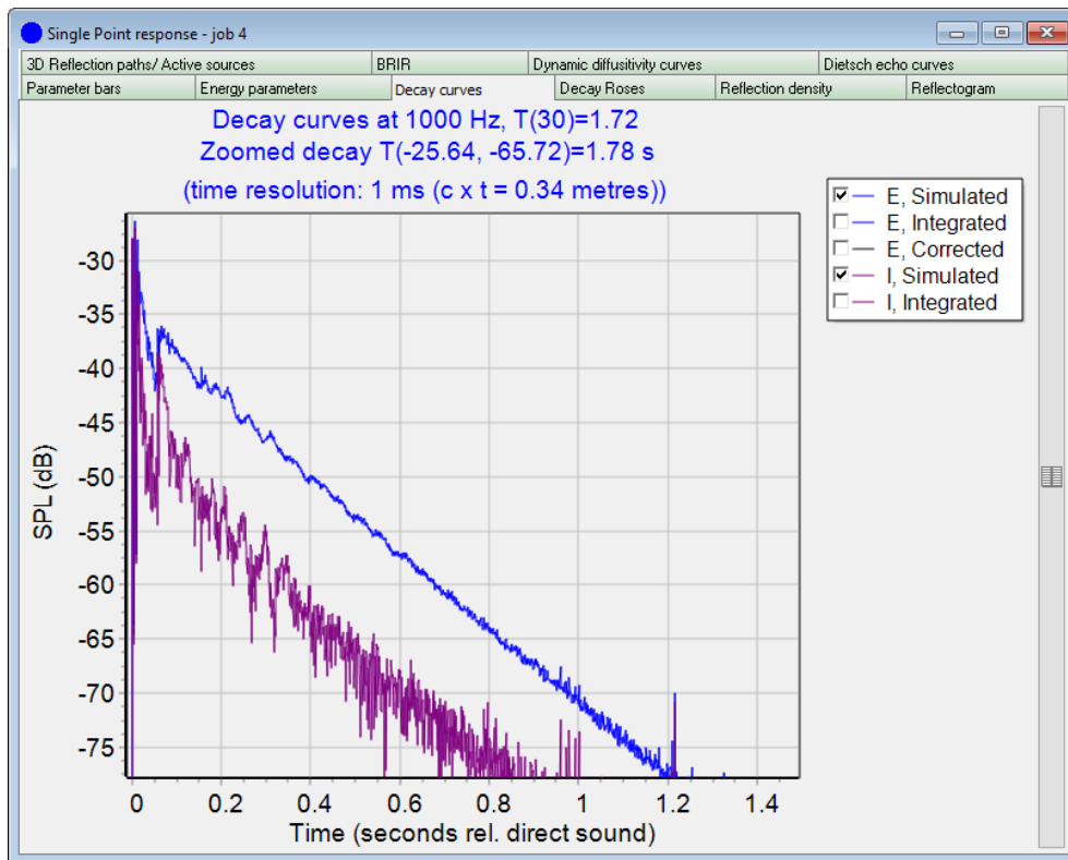
Figure 2: Energy and Intensity decay in Condition 1 (Reflective surfaces).
