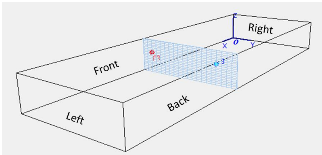
Figure 1: A rectangular room in ODEON with dimensions L*W*H = 30 \text{ m} * 10 \text{ m} * 3 \text{ m} . A source and a receiver are placed in the same YZ plane to study flutter echoes. The walls are named according to the receiver, which is facing the source.
